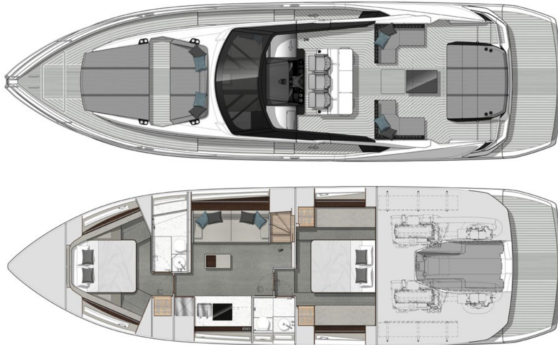
MAIN AND LOWER DECK SHOWN WITH OPTIONAL TENDER
