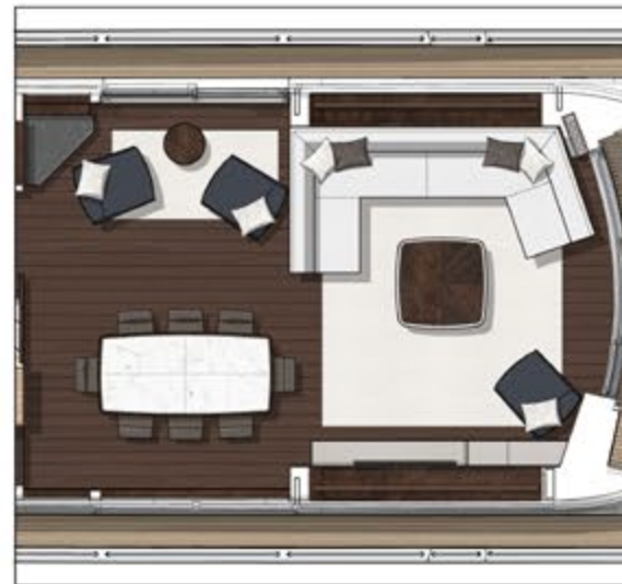
MAIN DECK OPTION SHOWN WITH ALTERNATIVE SALOON AND DINING ARRANGEMENT
