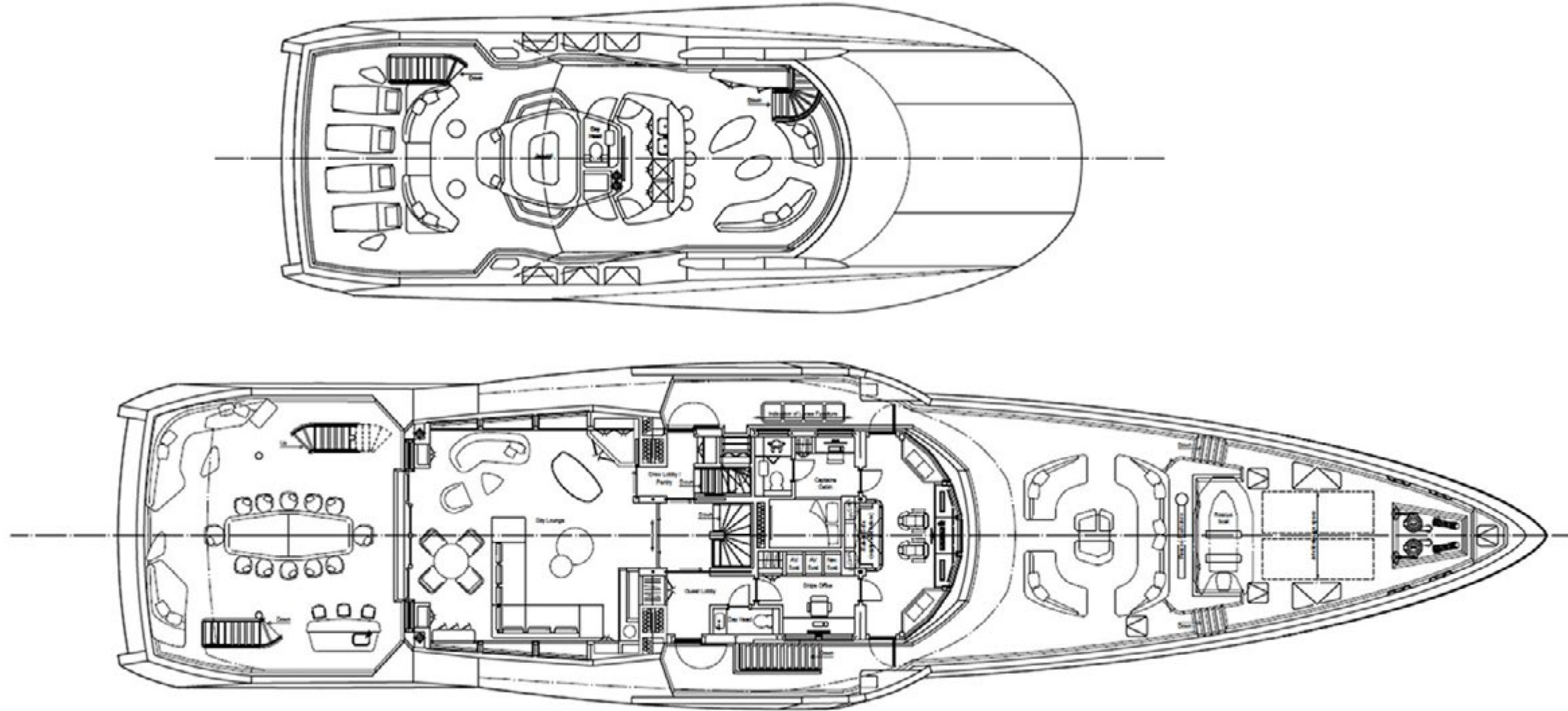
SUN AND WHEELHOUSE DECK
